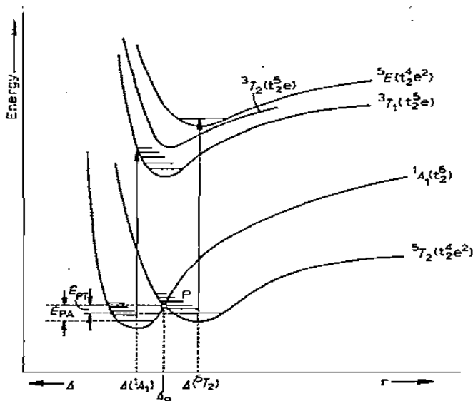
Fig. 1. Schematic potential energy curves for the lowest molecular states of a d^6 complex ion with almost equi-energetic ground states {}^5T_2 and {}^1A_1 (the lowest electronic transitions {}^5E \leftarrow {}^5T_2 and {}^3T_1 \leftarrow {}^1A_1 observed in the optical spectra are indicated).
