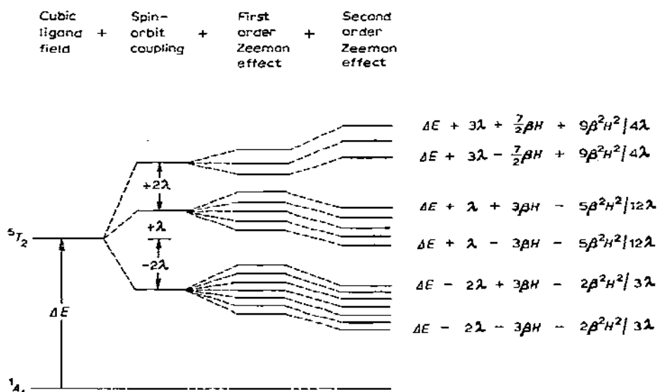
Fig. 2. Energy levels of a d^6 complex ion with close-lying ground states 5T_2 and 1A_1 in an octahedral field under the action of spin-orbit coupling, first and second order Zeeman effect. The energy expressions for the outermost final levels are indicated on the right hand side.
